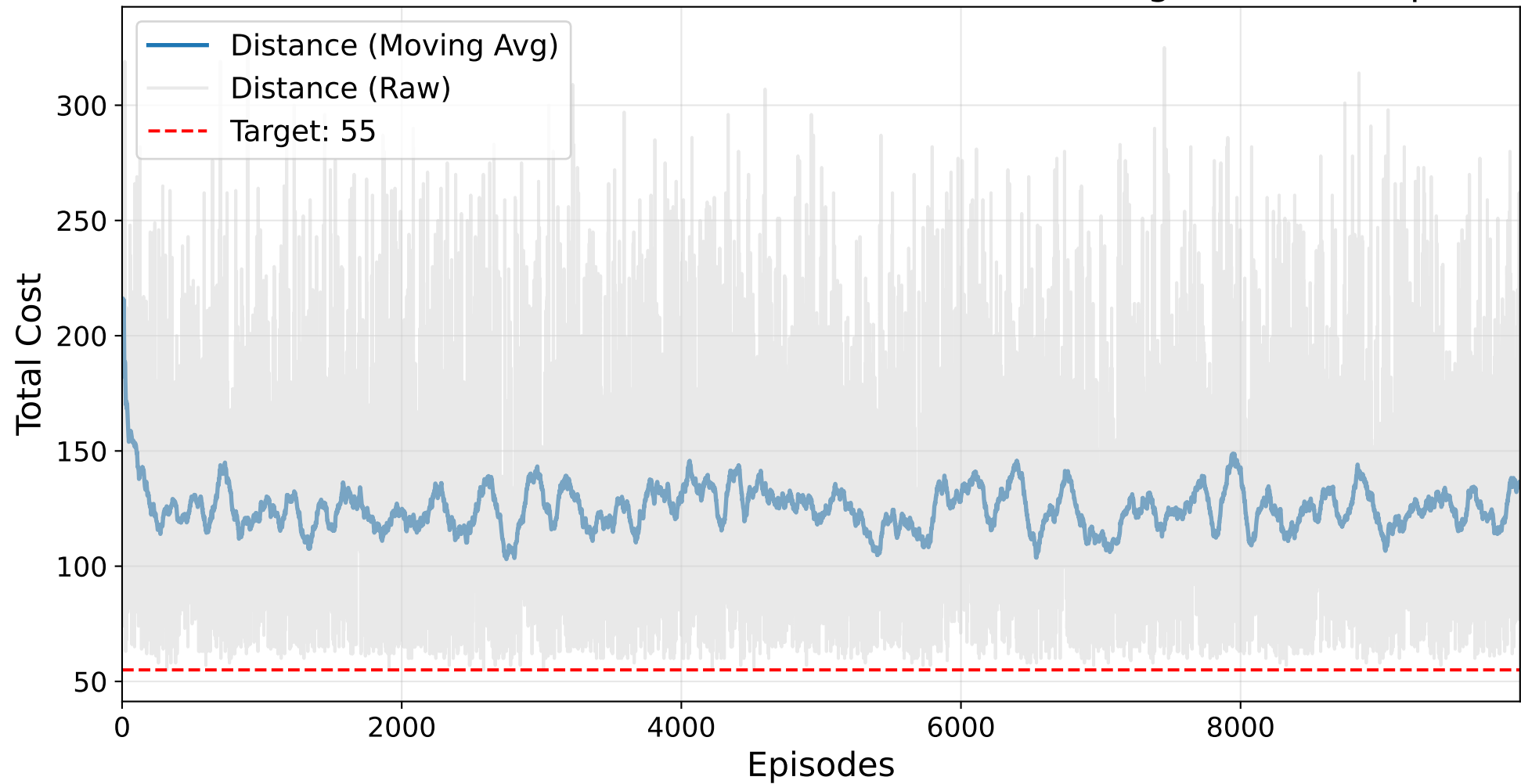
Final HYPERBAND TPE Masked AutoRL-SOP Training - br17.10.sop
